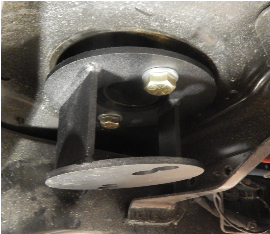
Upper Air Bag Mount Shown Installed
