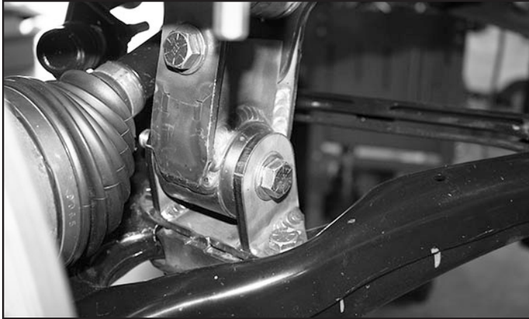
FIGURE 61 - STEP 38
