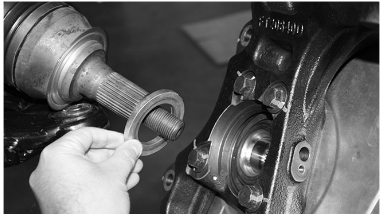
FIGURE 64 - STEP 41
