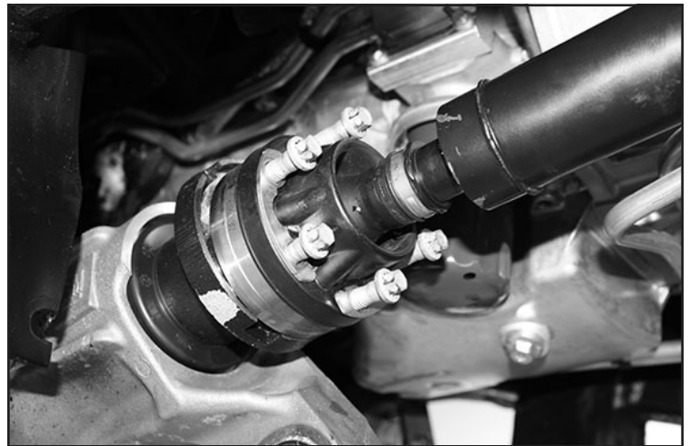
FIGURE 43 - STEP 27
