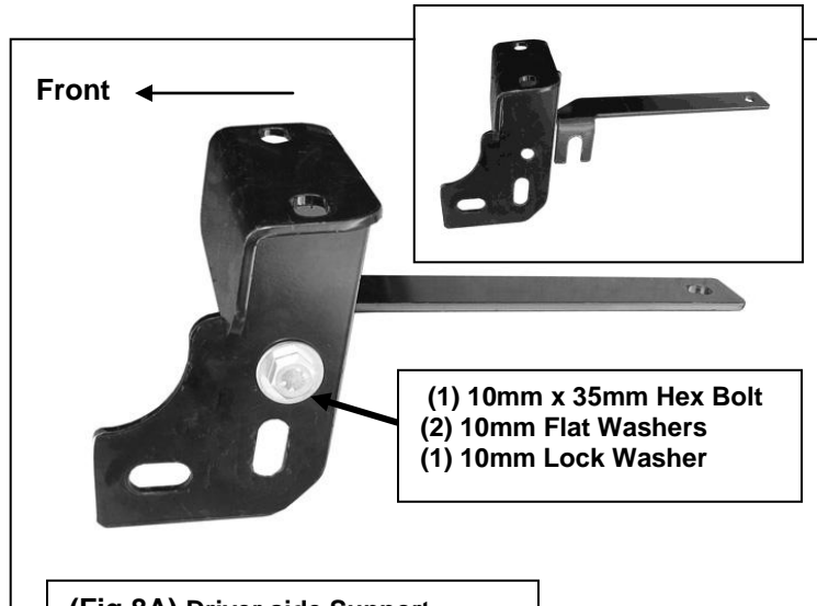
(Fig 8A) Driver side Support Bracket in "no Tow Hook" position
