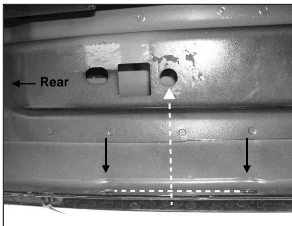
(Fig 3) 2007-10 driver side rear mounting location pictured. Locate the holes in the pinch weld to determine correct hole for 10mm Nut Plate
