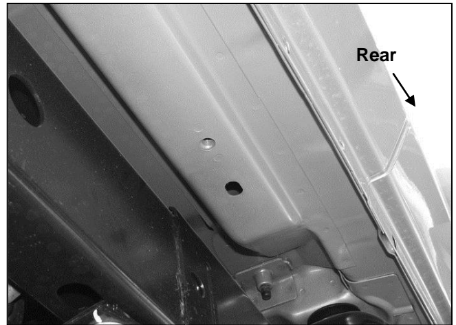
(Fig 2) Example of 2010-13 "closed" floor panel with threaded hole-10mm Nut Plate not required
