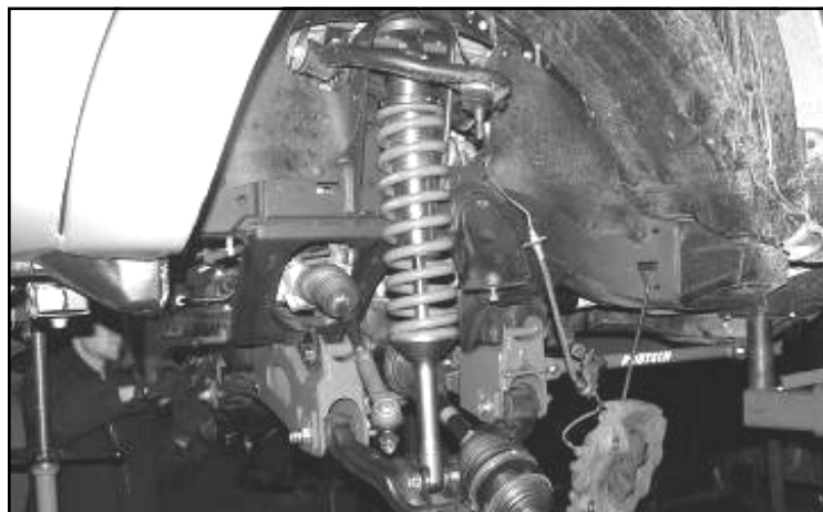
FIGURE 26 - STEP 30
