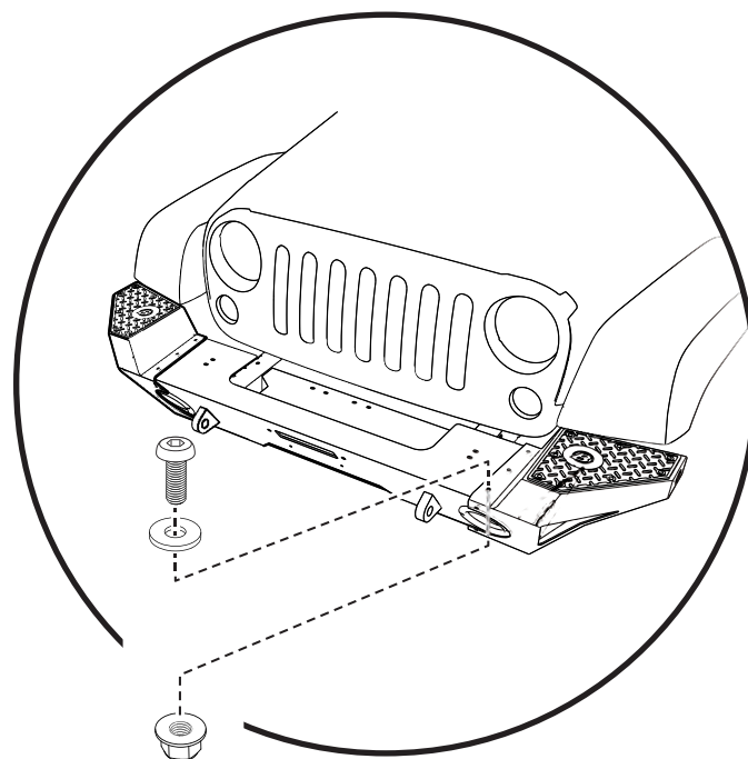
M8-1.25x25 Button Head Socket Screw Part #413.69 Qty. 6 per End Cap
