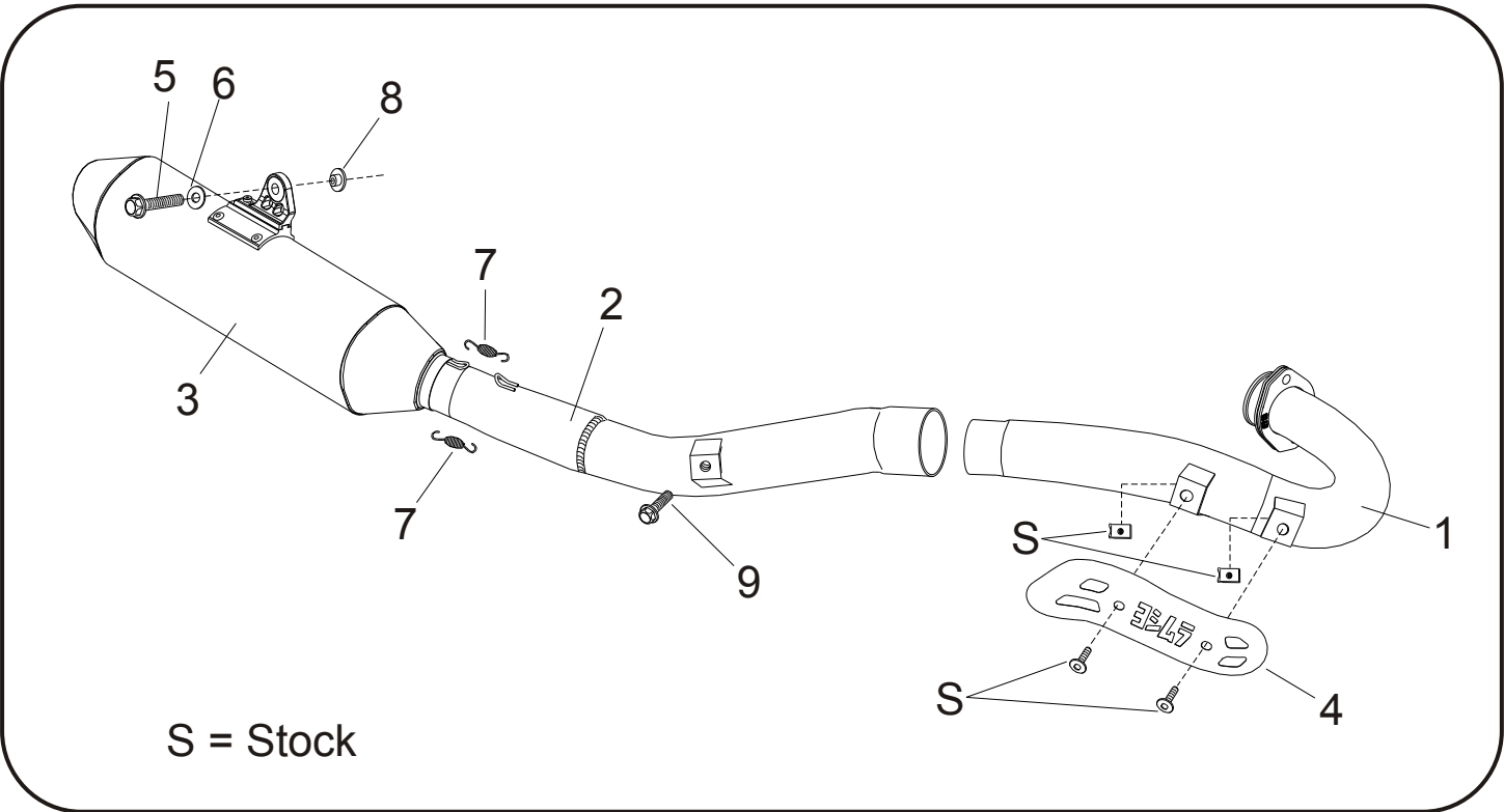
Parts Diagram
