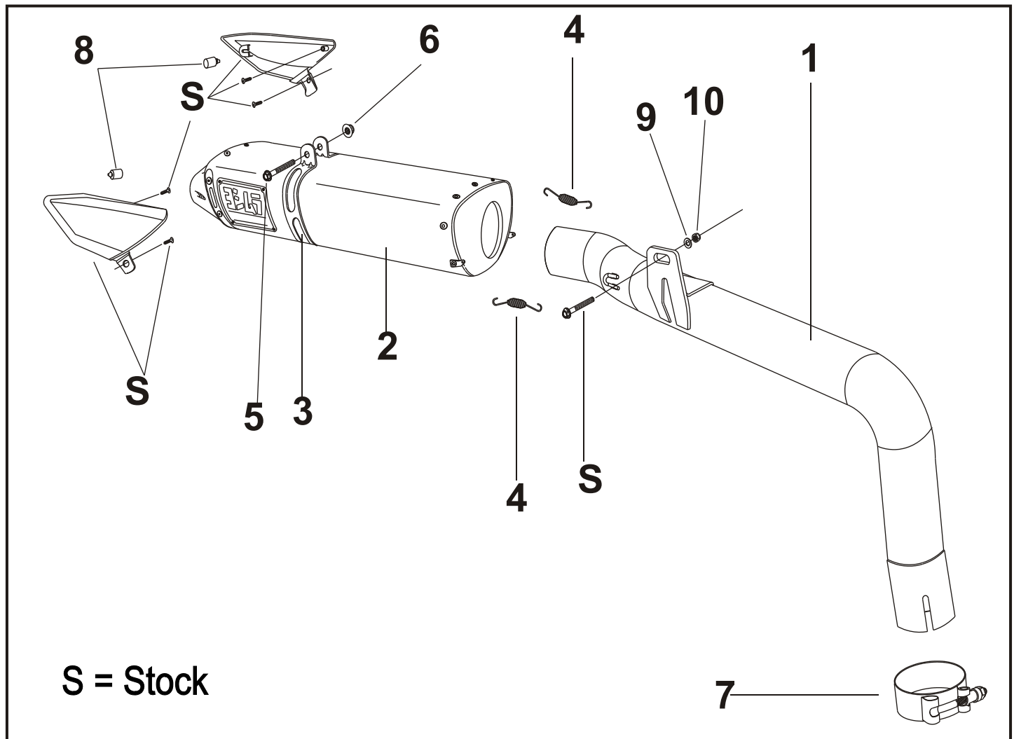
Parts Diagram
