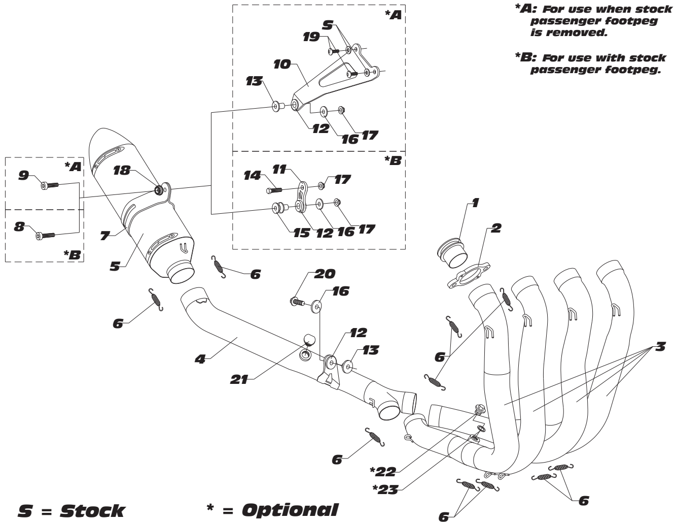
Parts Diagram
