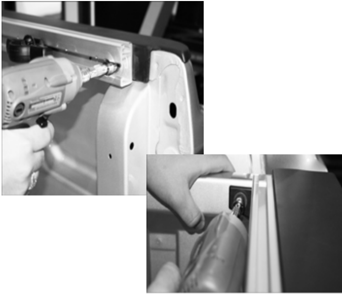
Cargo rails are held on by adhesive back tape and plastic fasteners.
